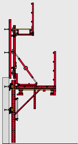
Use of the RCS CL on the first casting segment.
